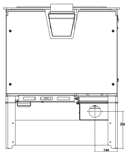
REAR ELEVATION
